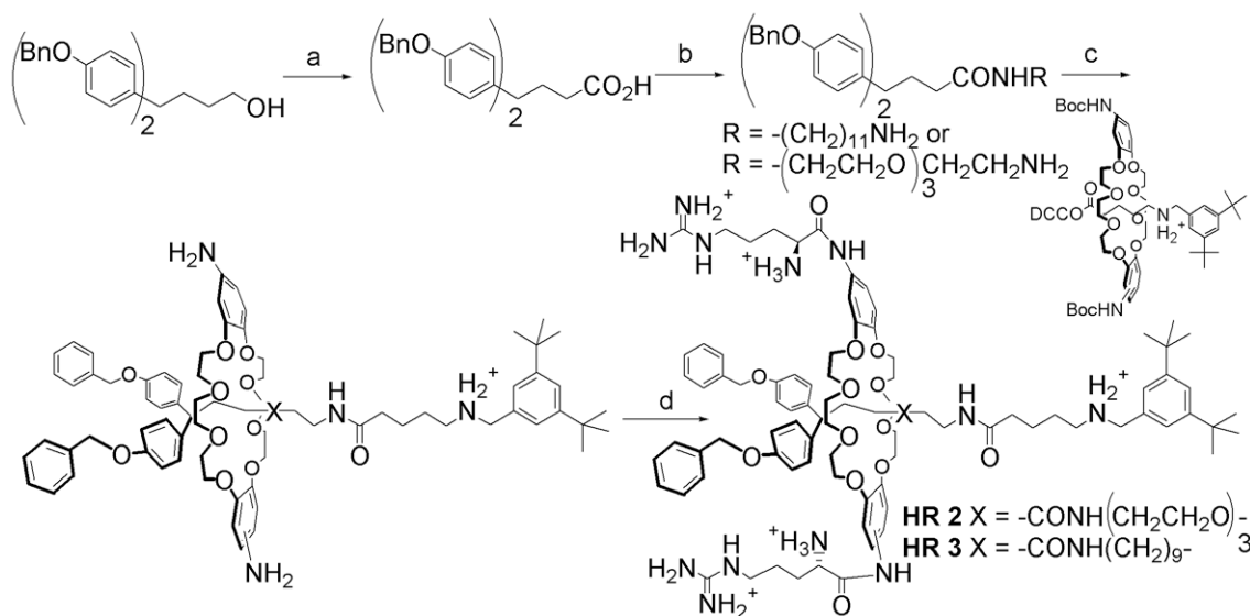
Scheme 1. Reagents and conditions: (a) \text{Na}_2\text{Cr}_2\text{O}_7 , \text{H}_2\text{SO}_4 , \text{H}_2\text{O} (88%); (b) i— \text{ClCOCl} , \text{Et}_3\text{N} , \text{CH}_2\text{Cl}_2 ; ii— \text{H}_2\text{N}(\text{CH}_2)_{11}\text{NH}_2 , DMSO or \text{H}_2\text{N}(\text{CH}_2\text{CH}_2\text{O})_3\text{CH}_2\text{CH}_2\text{NH}_2 , \text{CH}_2\text{Cl}_2 (33%, 73%); (c) i— \text{CHCl}_3 (65%, 42%); ii—TFA, \text{CH}_2\text{Cl}_2 (96%, 84%); (d) i— (\text{Boc})_3\text{ArgOH} , \text{HOBt} , \text{DCC} (68%, 56%); ii—TFA, \text{CH}_2\text{Cl}_2 (96%, 90%).
