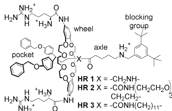
Figure 1. Host-rotaxanes used in this study and their components.
